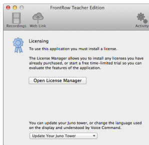
Mac OS
